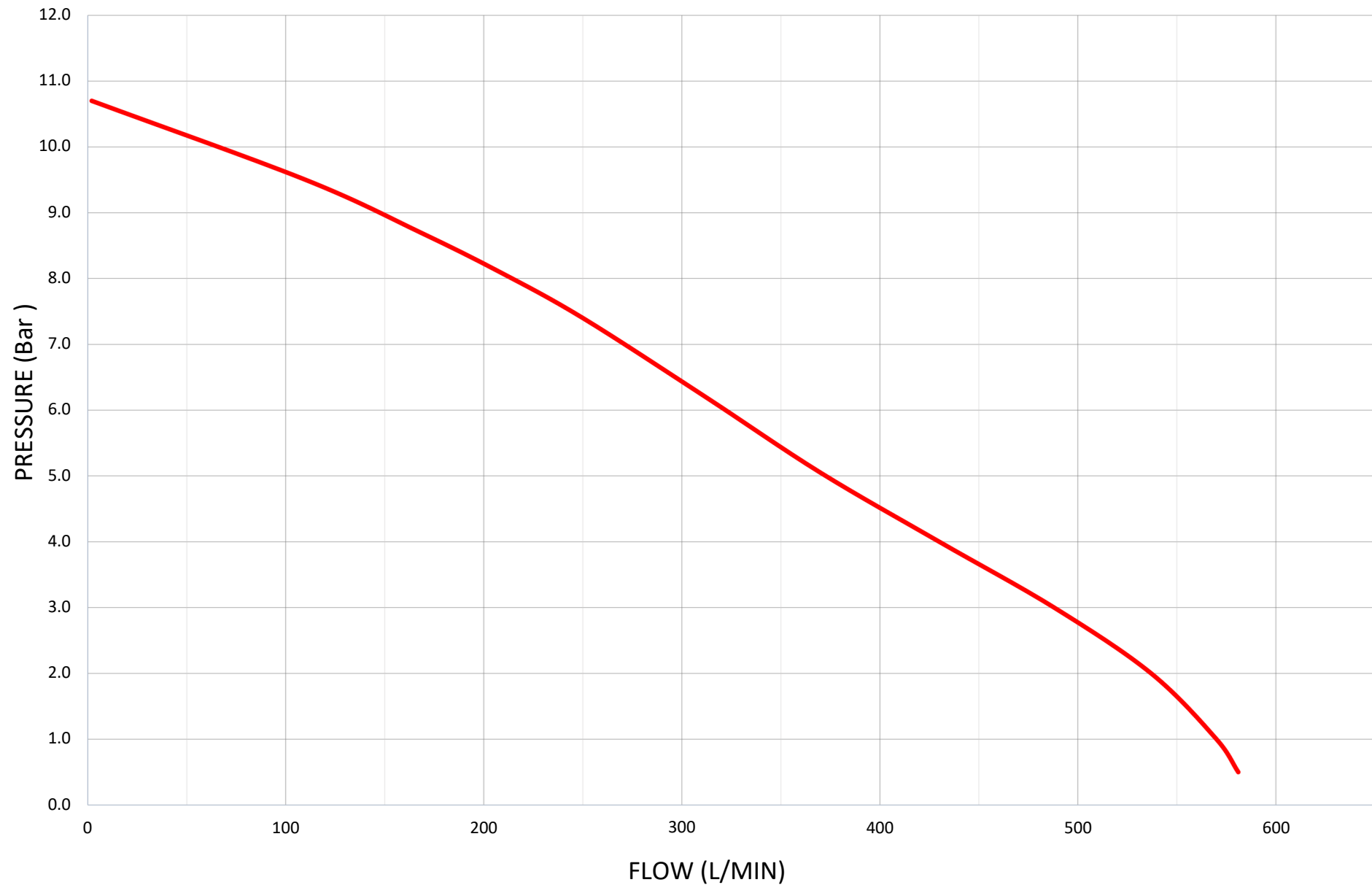
Typical Performance of FTP -400-D at NTP Conditions
