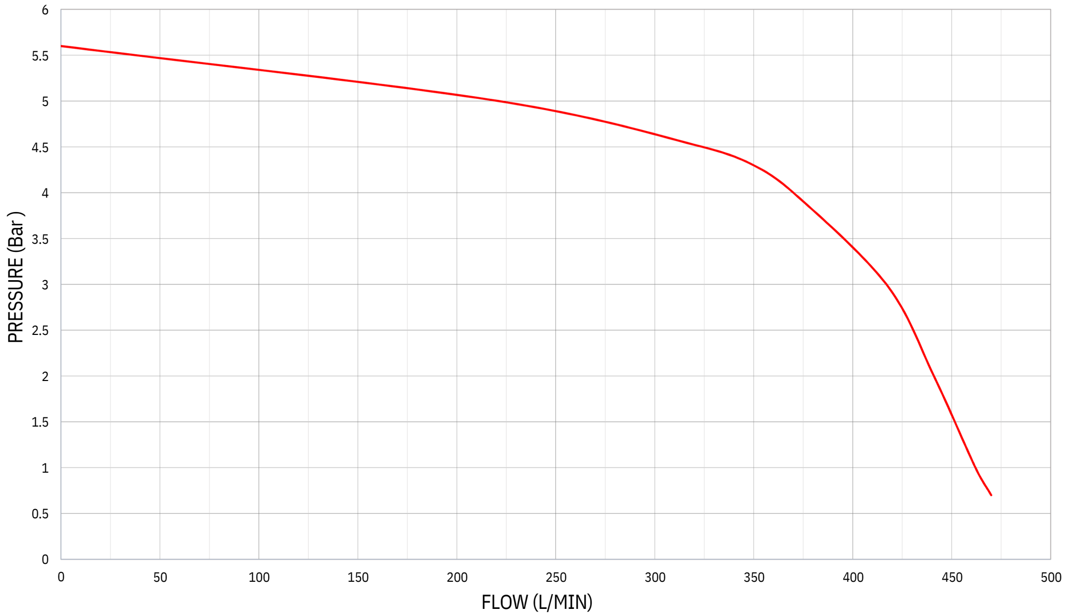
Typical Performance of FTP-275-P
