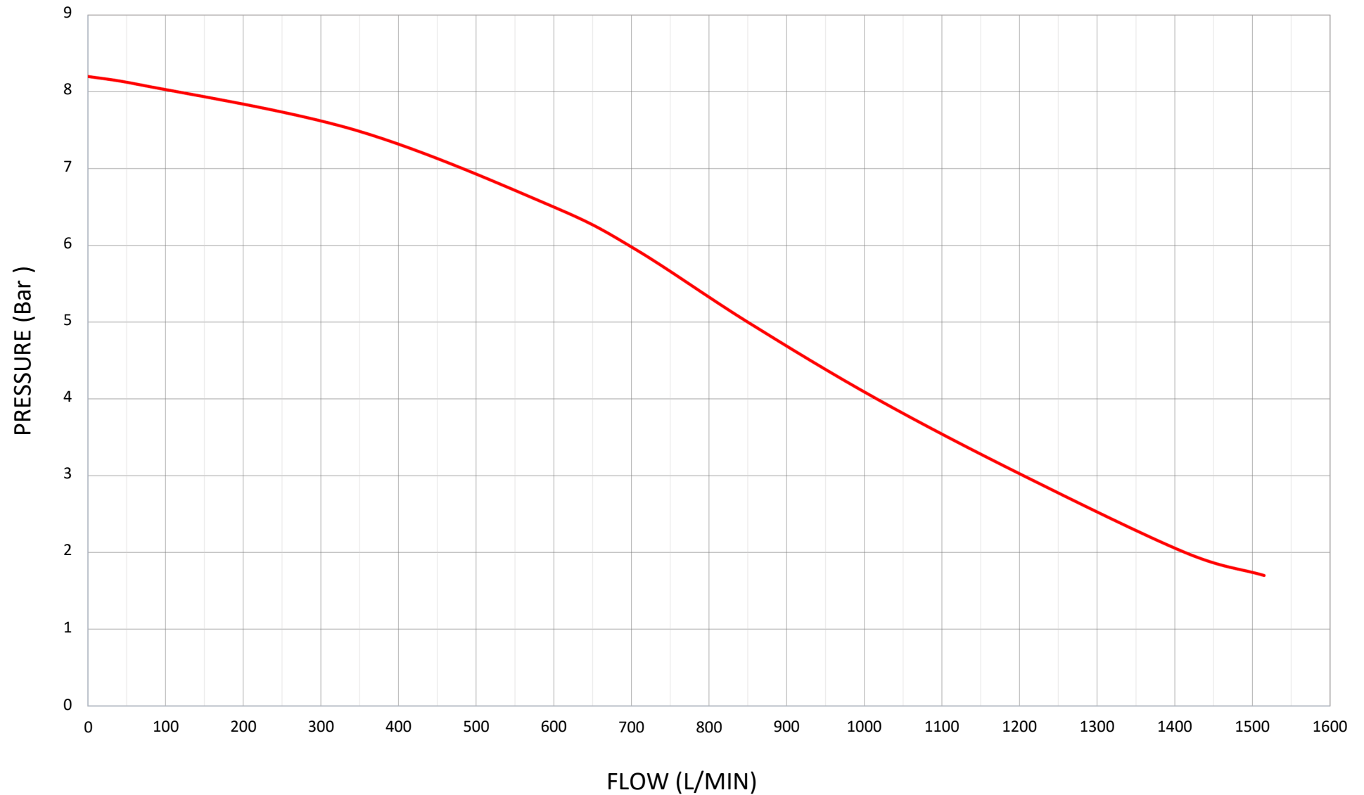
Typical Performance of FTP-800-P at NTP Conditions
